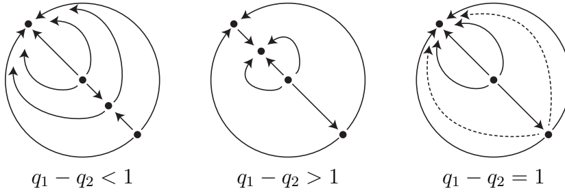
FIGURE 5. Phase portraits on the Poincaré disk for normal form (i) in Proposition 6.2 with \lambda > 0 . The dashed line in the case q_1 - q_2 = 1 indicates a parabolic sector at the infinite equilibrium \theta = -\pi/4 that may or may not exist.
