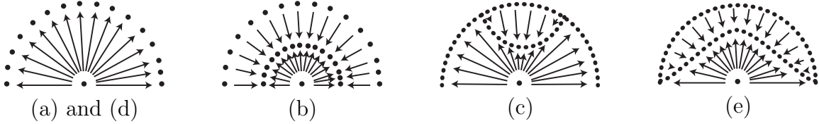
FIGURE 15. Phase portraits with \tilde{\lambda} > 0 for normal form (X) in Proposition 6.3, when all points at infinity are equilibria. Cases (a)–(e) as in Lemma 6.4. Conventions as in Figure 10.
