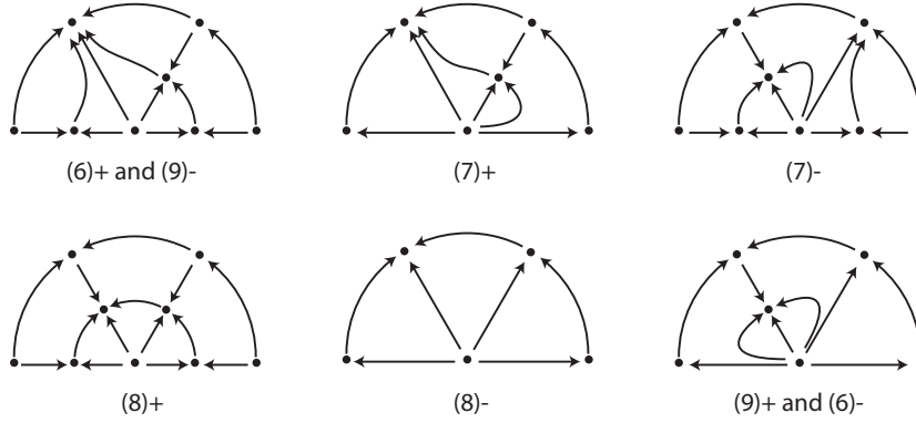
FIGURE 11. Phase portraits for normal form (V) in Proposition 6.3 for \tilde{\lambda} > 0 when Q_1 and Q_2 have no common factor. Each diagram in [8][Figure 5.1] gives rise to two cases, depending on the choice of sign, numbering refers to their cases. Cases (6)\pm and (9)\mp coincide. The equator of the Poincaré sphere is a global attractor in case (8)- and there is a polycycle in case (8)+ . Conventions as in Figure 10.
