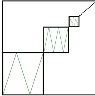
FIGURE 1. Graph of the map T_{a,b} .
