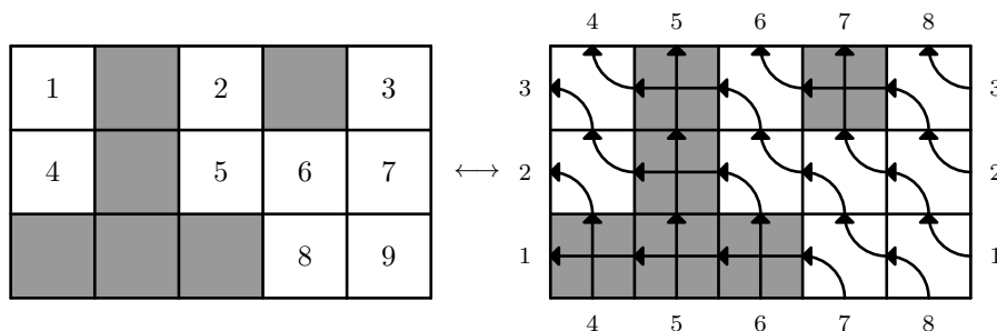
Figure 1: Labelled 3 \times 5 diagram (left) with pipe dream construction (right) associated to the diagram \{(1, 2), (1, 4), (2, 2), (3, 1), (3, 2), (3, 3)\} in \mathcal{O}_q(M_{3,5}(\mathbb{K})) .
