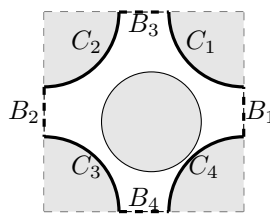
Fig 1.b Poincaré section (in bold)
